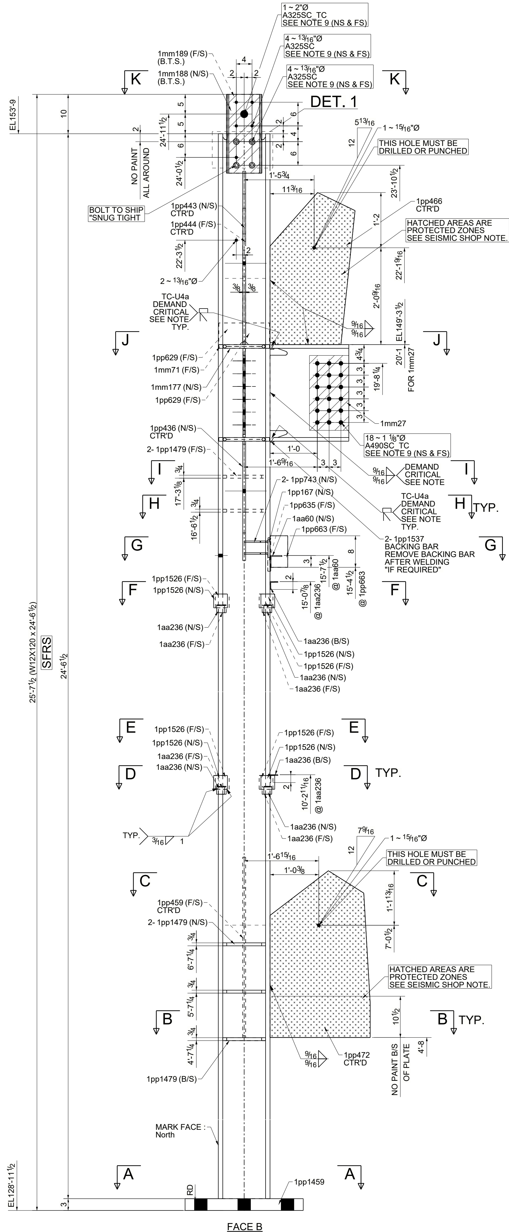
ONE - COLUMN - 1C62
