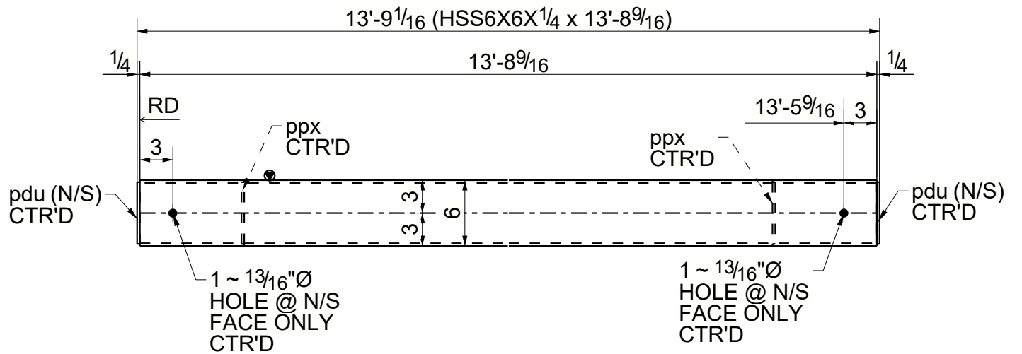
ONE - VERTICAL HSS BRACE - 125D2
