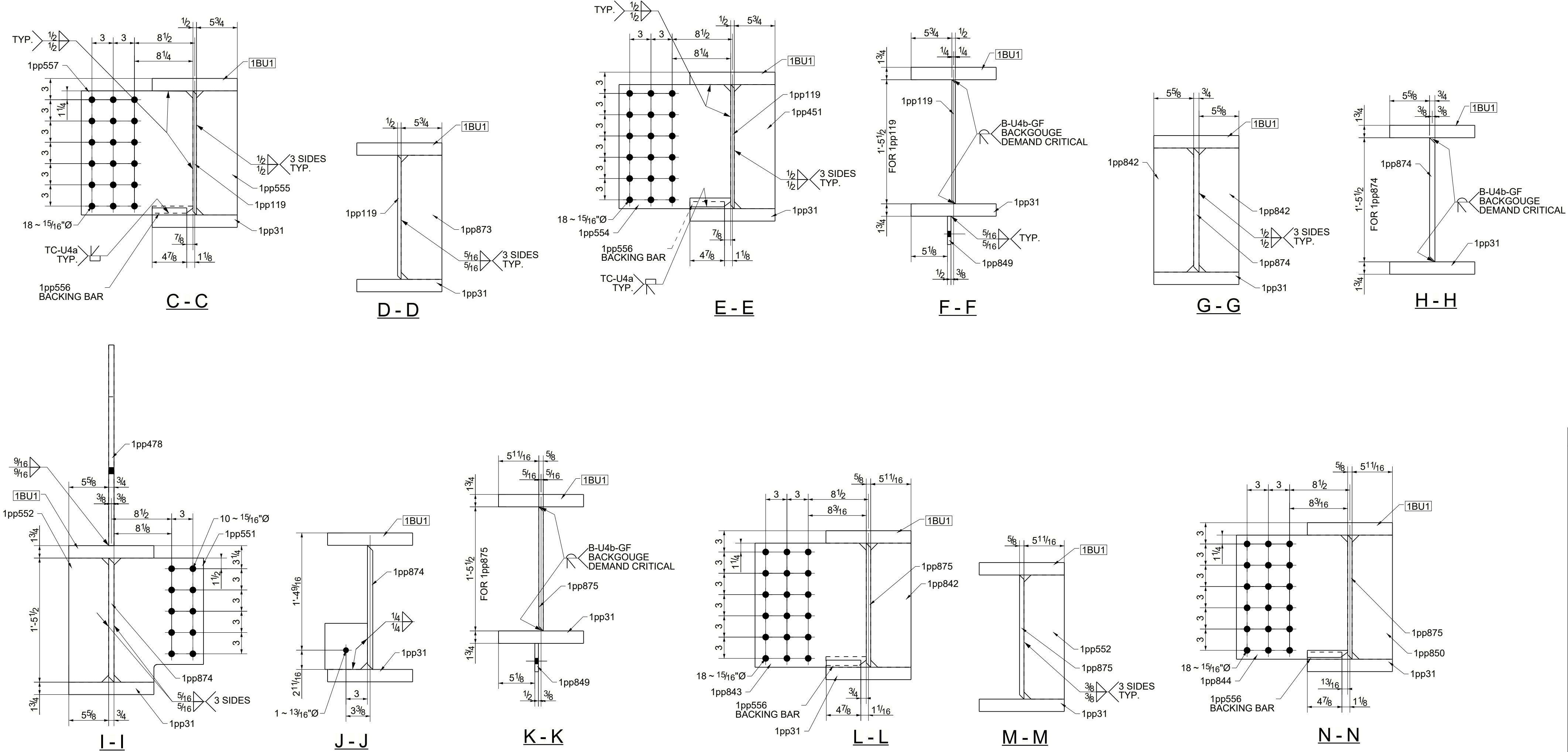
DETAIL OF 1BU1
