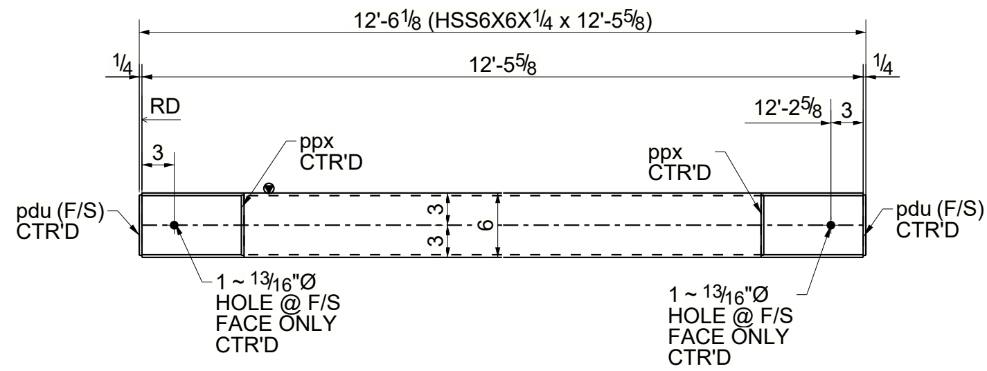
2 - VERTICAL HSS BRACE - 125D3
