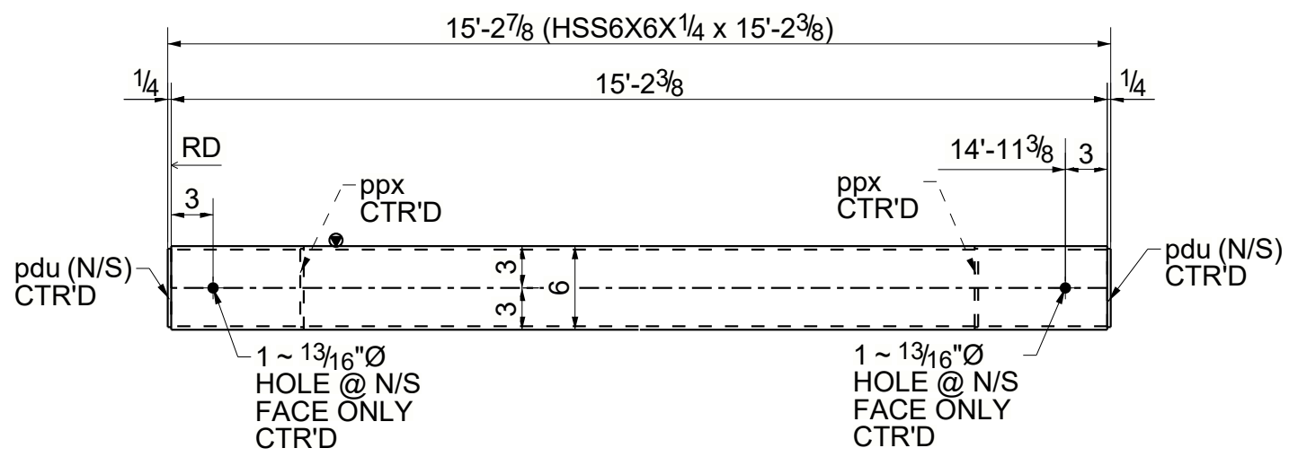
2 - VERTICAL HSS BRACE - 125D4
