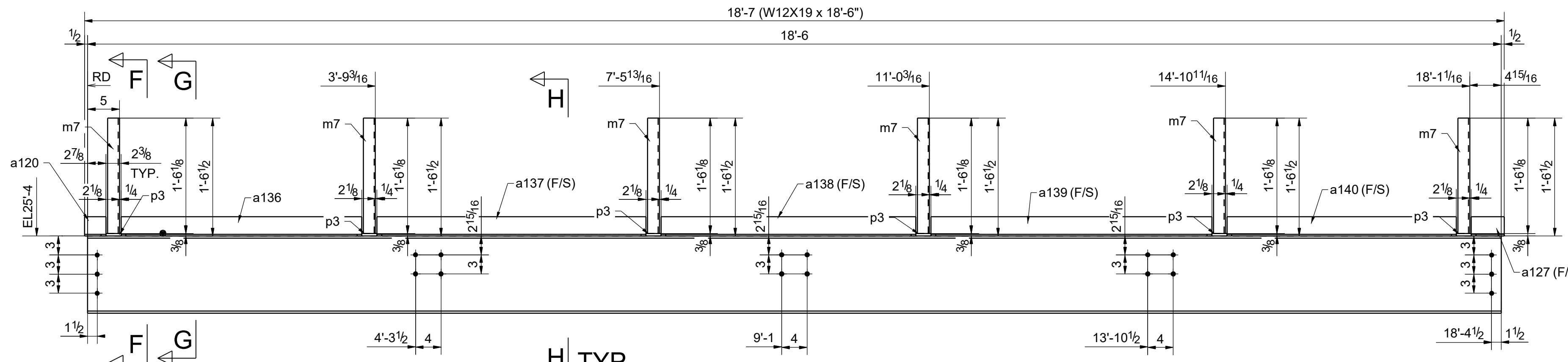
ONE - BEAM - 12B2
