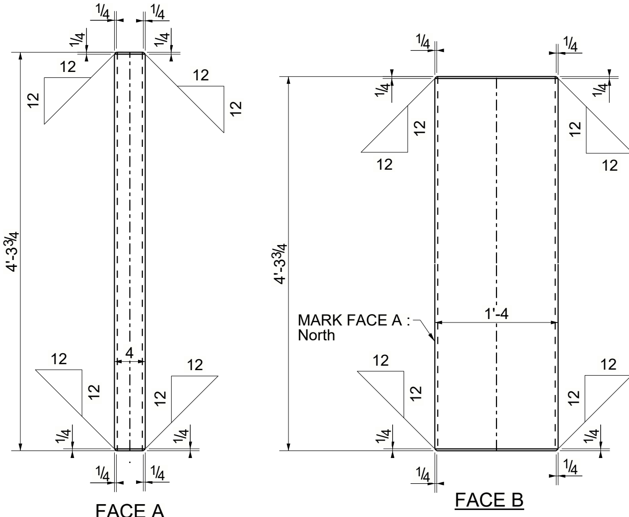
DETAIL OF 115C1
