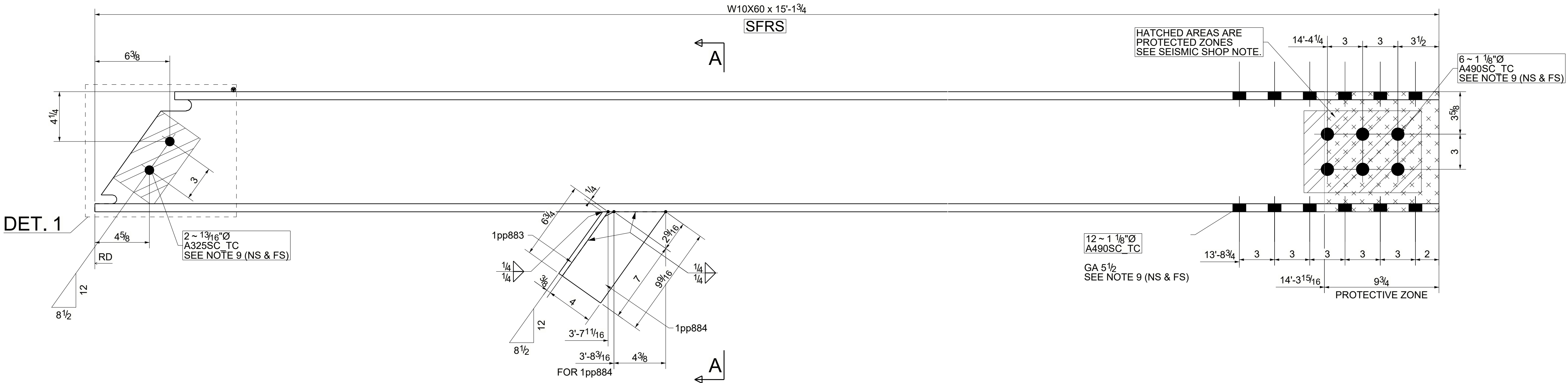
TOP VIEW
