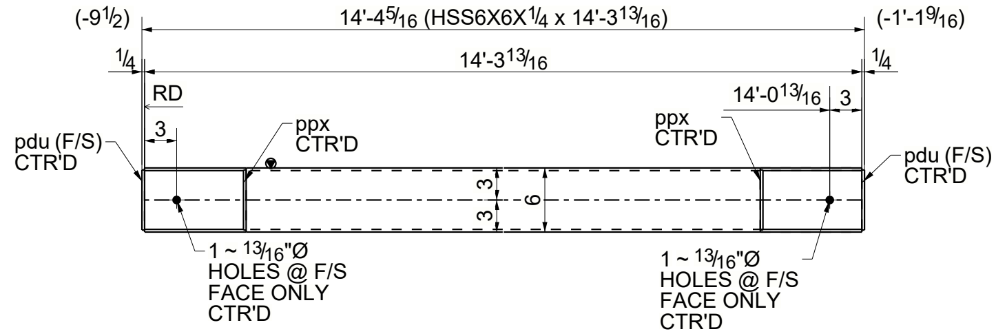
2 - VERTICAL HSS BRACE - 125D1
