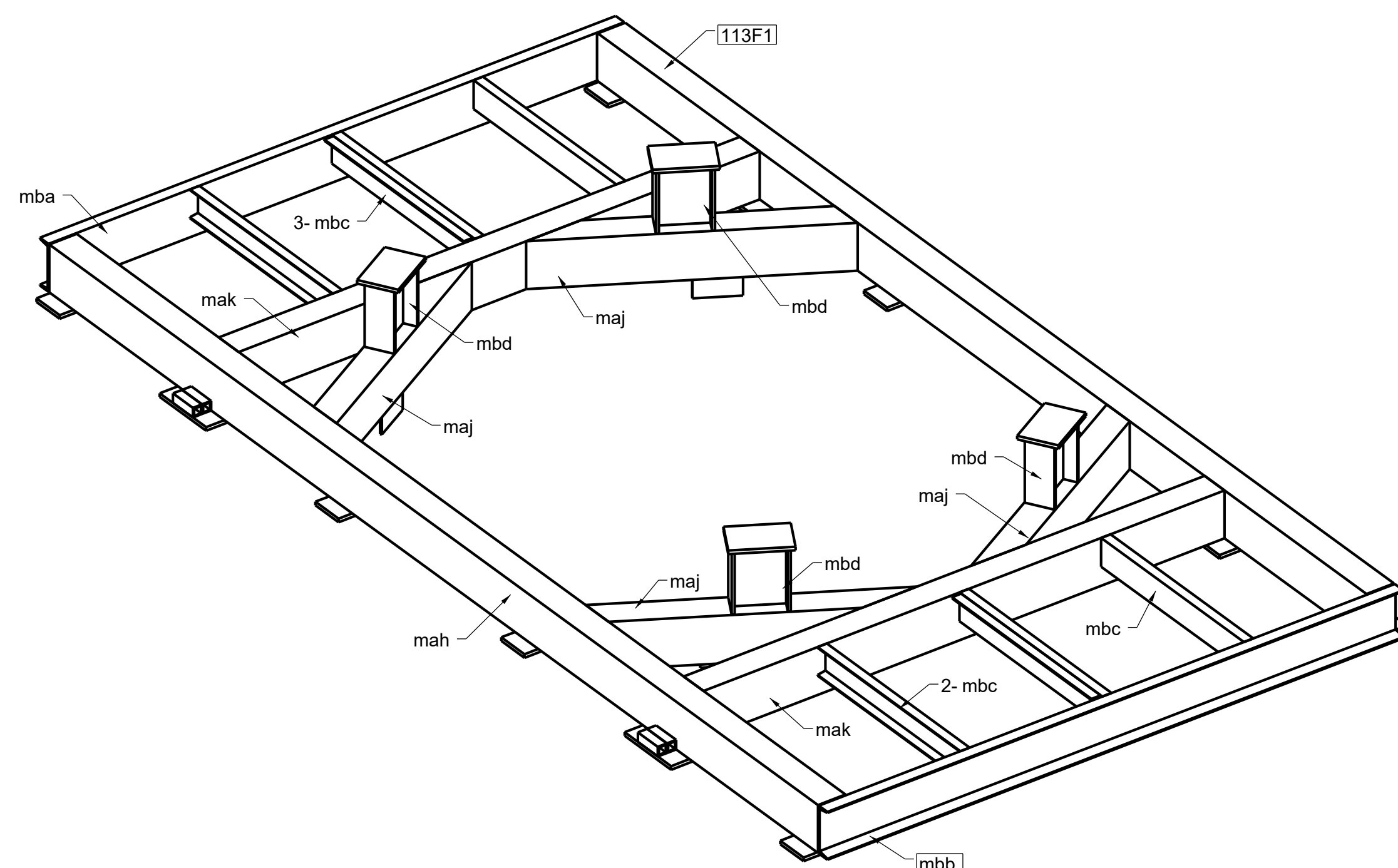
3D-VIEW OF 113F1
