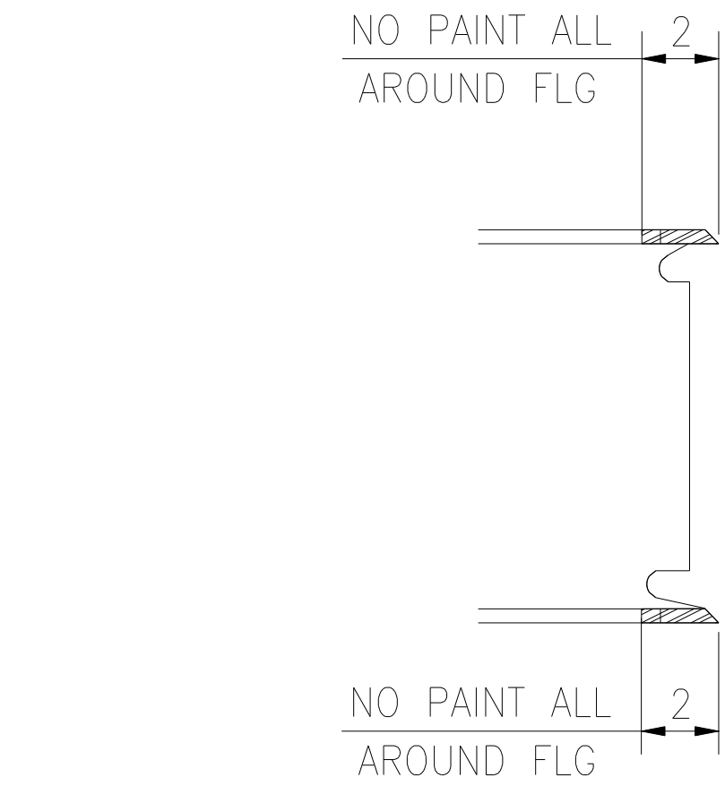
TYP PAINT BLOCK DETAIL @ MOMENT PREP BRACE END
